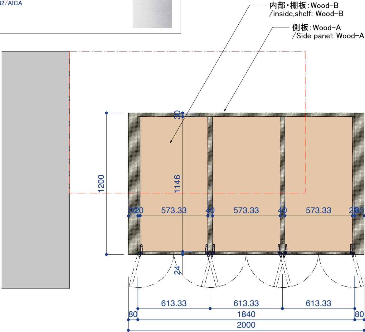
section A
