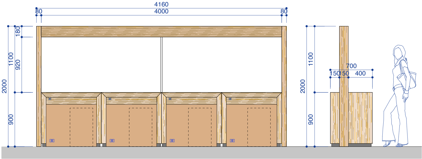
Booth unit C x1
