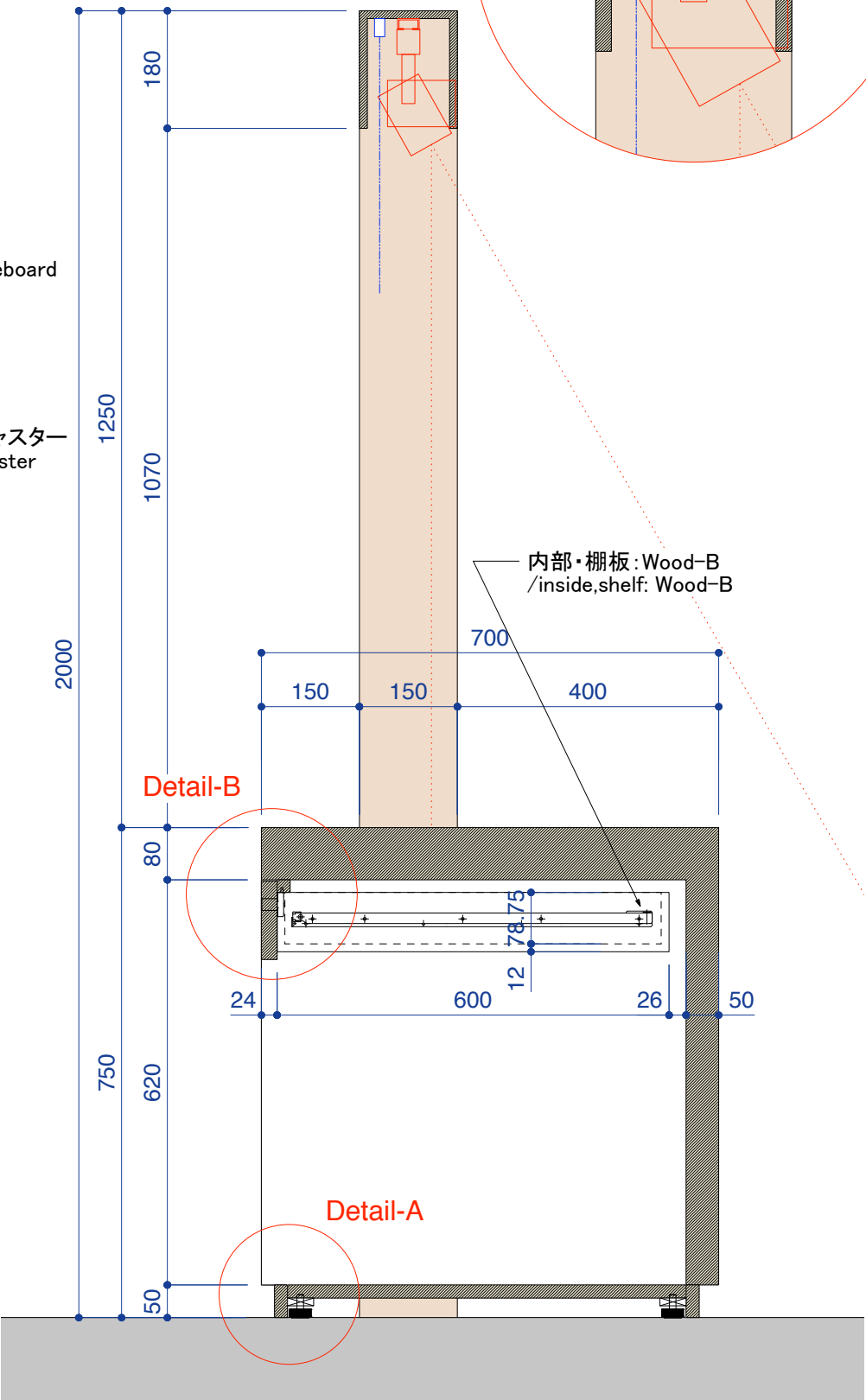
section A scale:1/10
