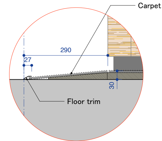
Floor Detail scale:1/8
