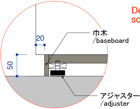
Detail-A scale:1/5
