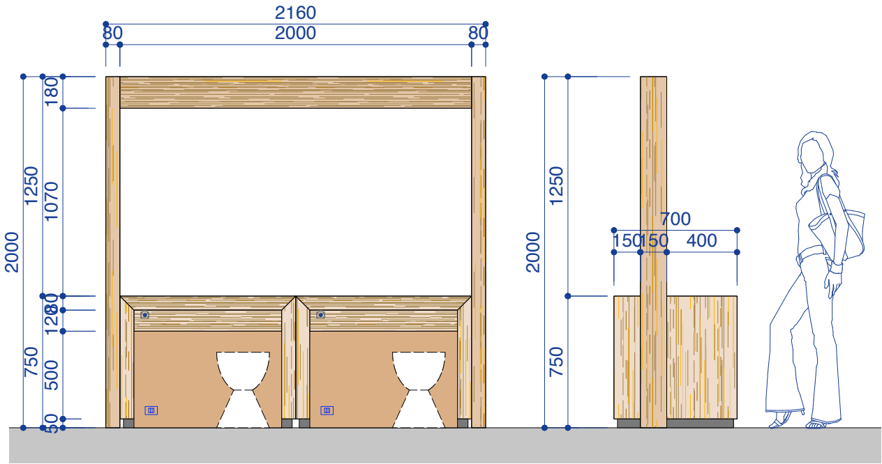
Booth unit A x1
