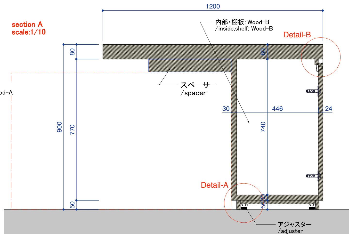
Detail-A scale:1/5
