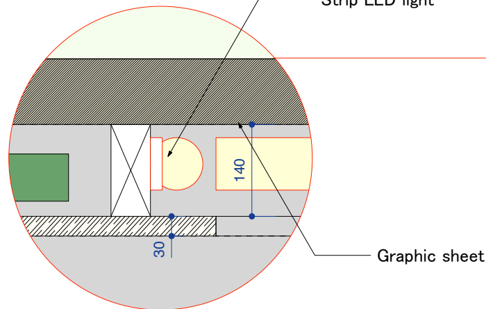
Wall Detail scale:1/8
